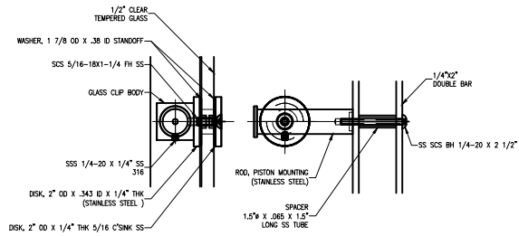
ROD-PISTON ASSEMBLY -END POST SCALE: 6" = 1'-0"
