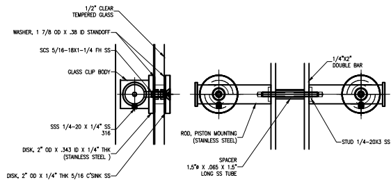
ROD-PISTON ASSEMBLY-INT POST SCALE: 6" = 1'-0"
