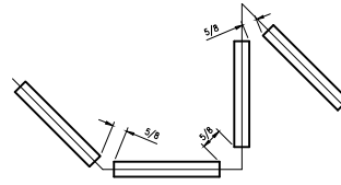
TYPICAL GLASS CORNERS DETAIL SCALE: 6" = 1'-0"
