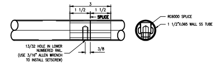
FACTORY CUT SPLICE SCALE: 6" = 1'-0"
